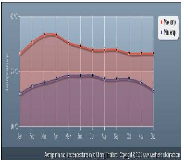
Average minimum and maximum temperature over the year
