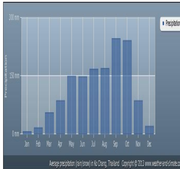
Average monthly precipitation over the year
